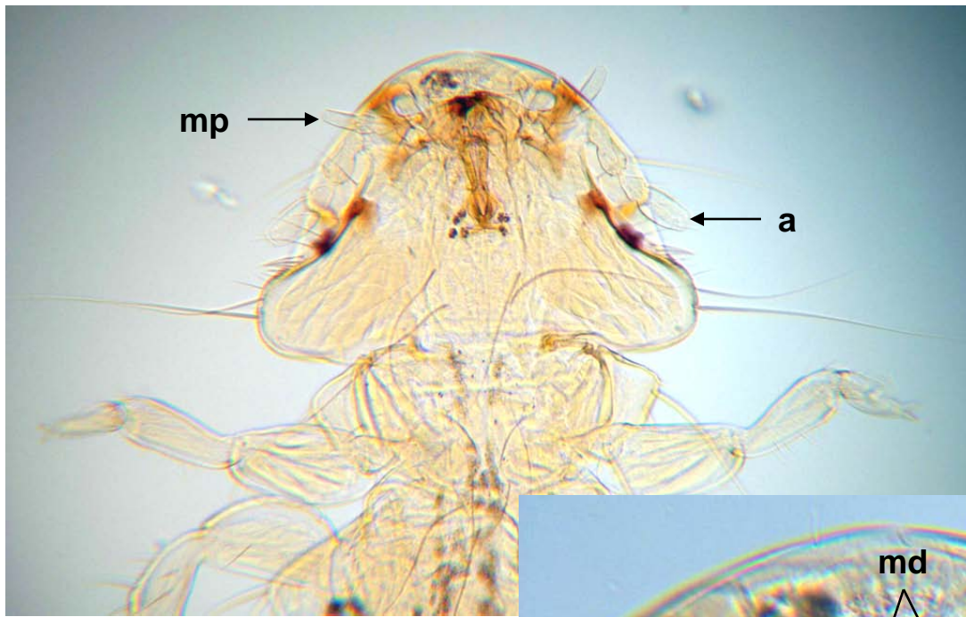
Menopon gallinae female (det. S. P. Koff).
